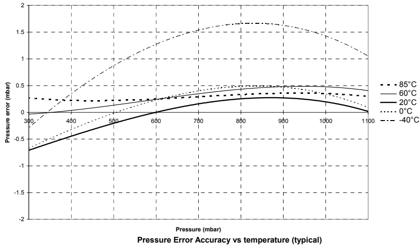
Pressure Error Accuracy vs temperature (typical)
